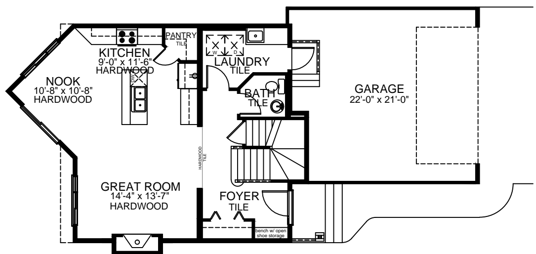
MAIN FLOOR PLAN - 757 SQ. FEET DEV.
