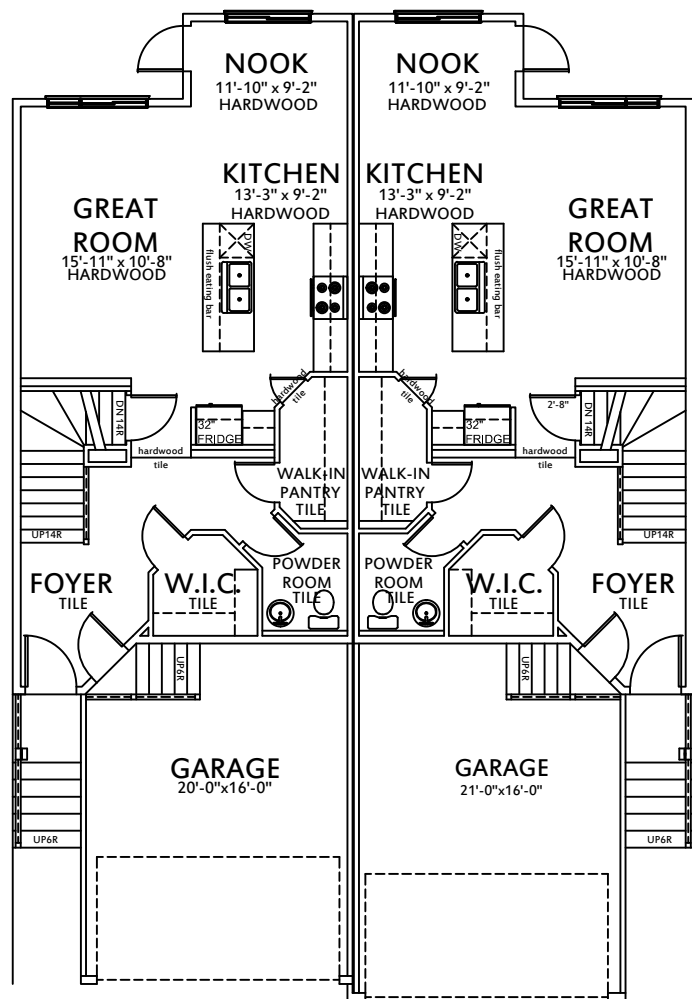
MAIN FLOOR PLAN - 707 SQ. FT. DEV. PER SIDE
