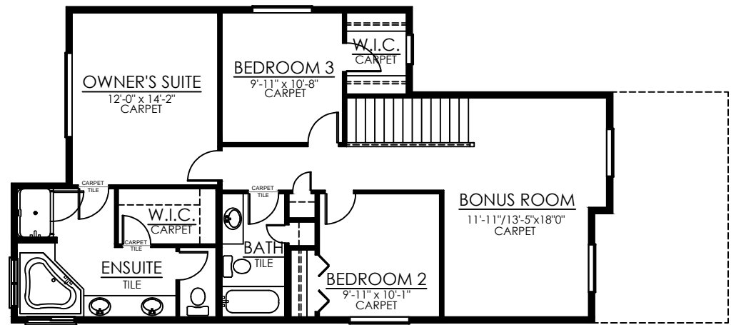
SECOND FLOOR PLAN - 1066 SQ. FT. DEV.
