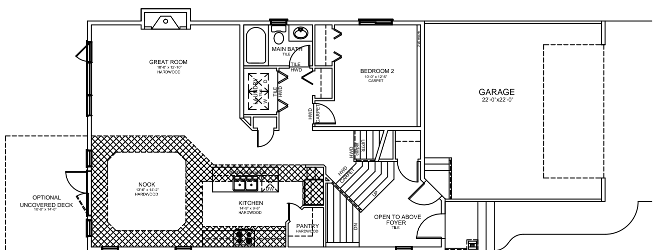
MAIN FLOOR PLAN - 1166 SQ. FEET DEV.
