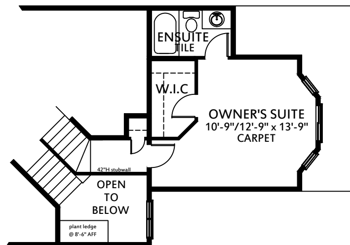
SECOND FLOOR PLAN - 344 SQ. FEET DEV.
