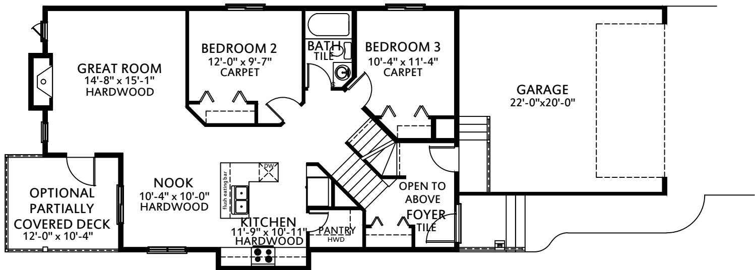
MAIN FLOOR PLAN - 1083 SQ. FEET DEV.
