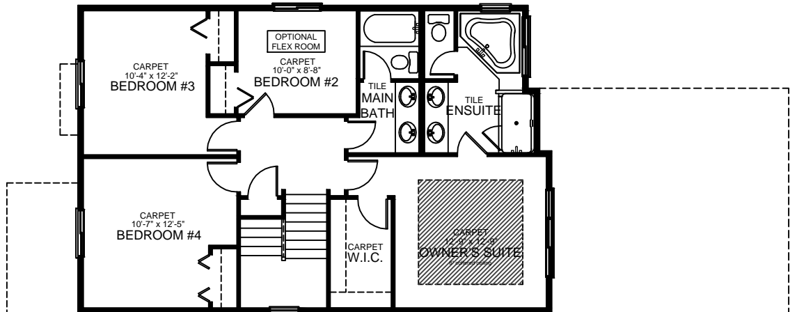
SECOND FLOOR PLAN - 955 SQ. FEET DEV.
