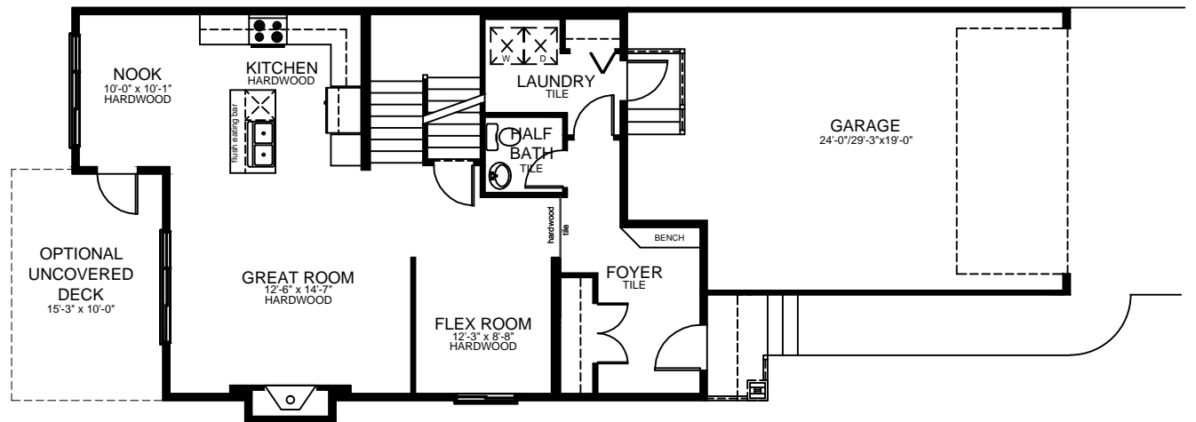
MAIN FLOOR PLAN - 927 SQ. FEET DEV.
