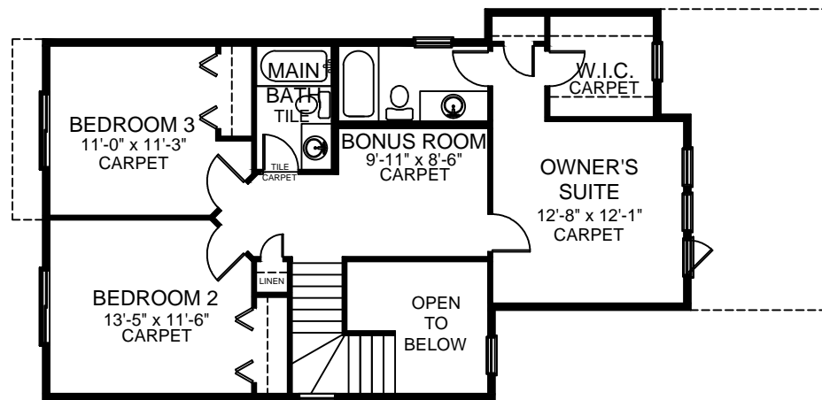
SECOND FLOOR PLAN - 844 SQ. FT. DEV.
