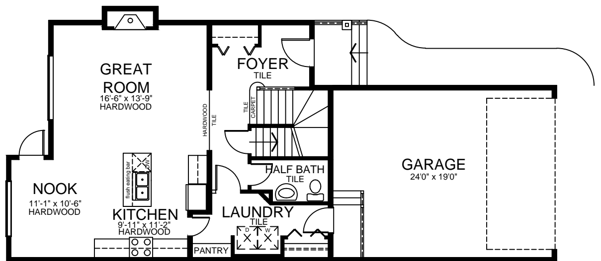
MAIN FLOOR PLAN - 831 SQ. FEET DEV.
