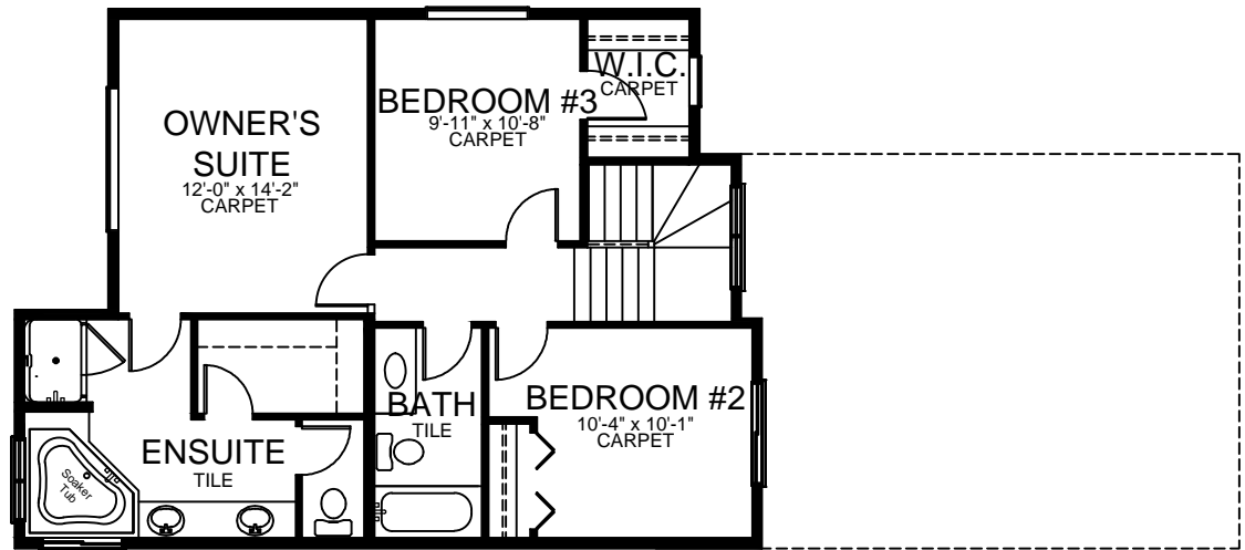
SECOND FLOOR PLAN - 783 SQ. FT. DEV.
