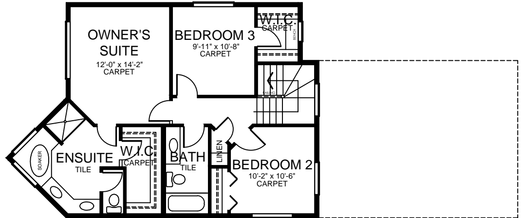
SECOND FLOOR PLAN - 778 SQ. FT. DEV.
