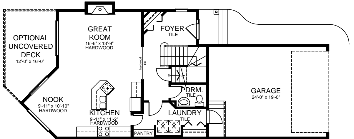
MAIN FLOOR PLAN - 832 SQ. FT. DEV.
