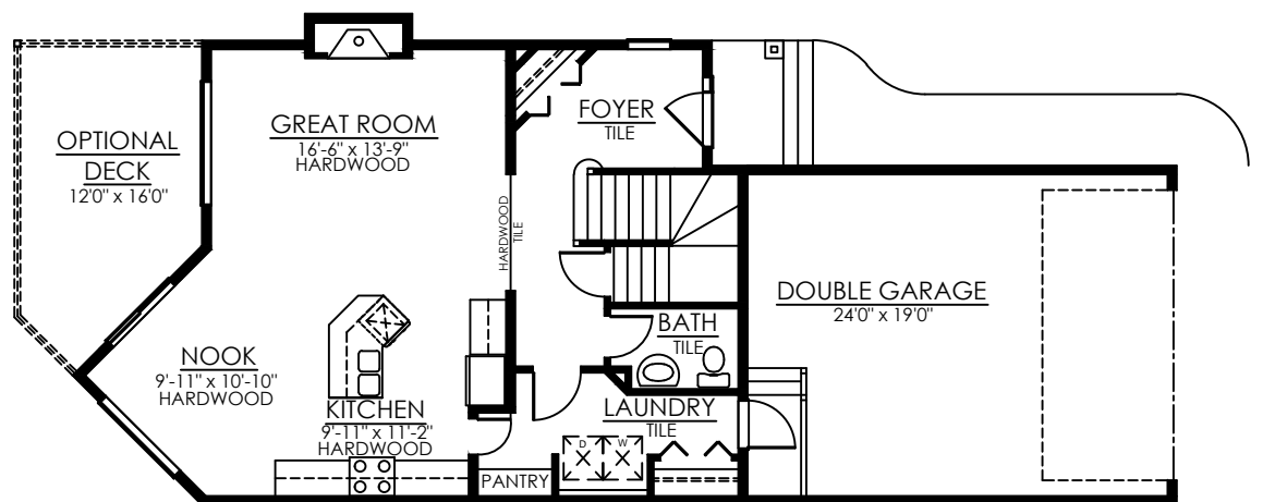
MAIN FLOOR PLAN - 831 SQ. FEET DEV.
