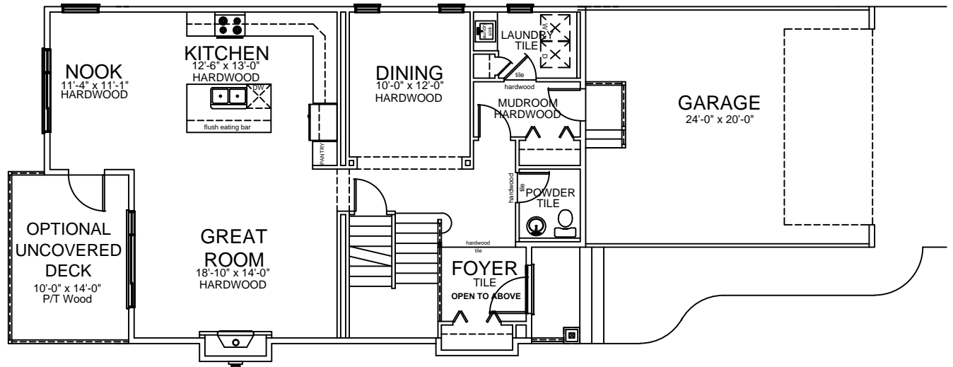
MAIN FLOOR PLAN - 1133 SQ. FT. DEV.
