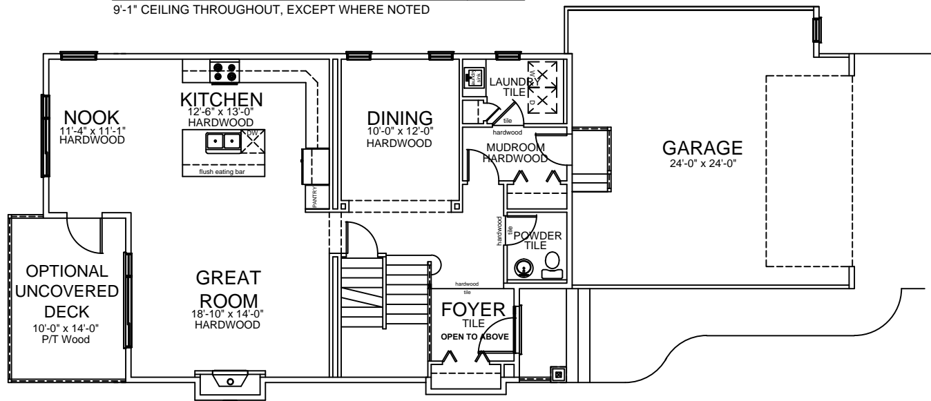
MAIN FLOOR PLAN - 1133 SQ. FT. DEV.
