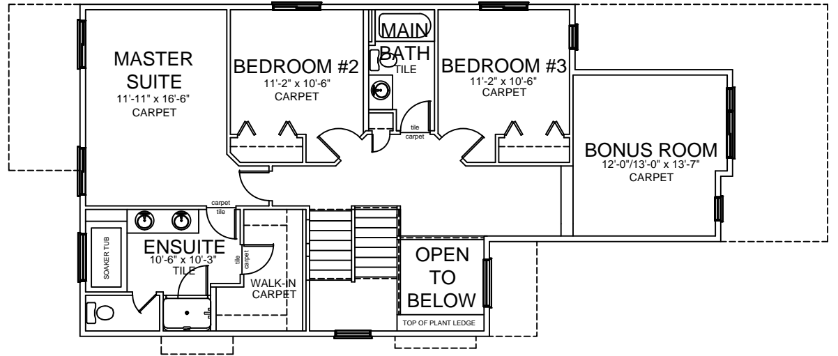
SECOND FLOOR PLAN - 1159 SQ. FT. DEV.
