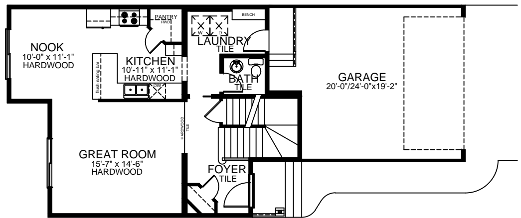
MAIN FLOOR PLAN - 783 SQ. FT. DEV.
