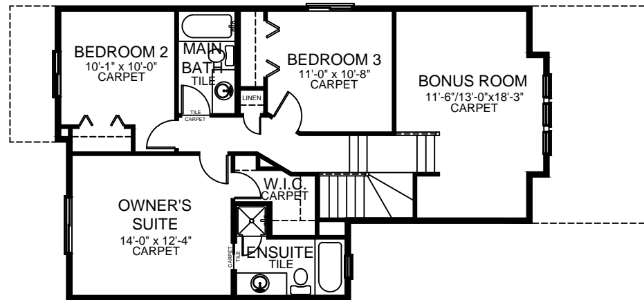
SECOND FLOOR PLAN - 933 SQ. FT. DEV.
